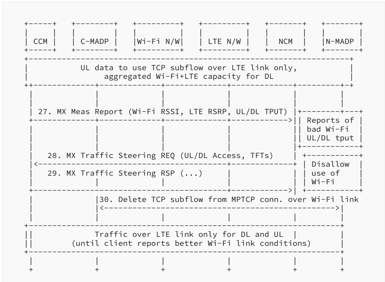
Figure 21: MAMS-Assisted MPTCP Proxy as User Plane - Part 4
