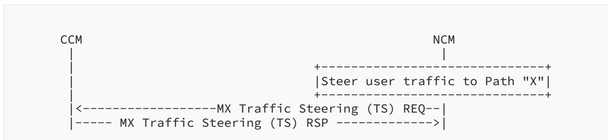
Figure 9: MAMS Traffic-Steering Procedure
