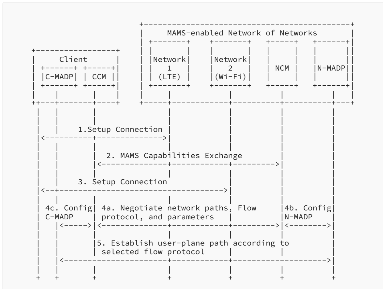
Figure 16: MAMS Call Flow
