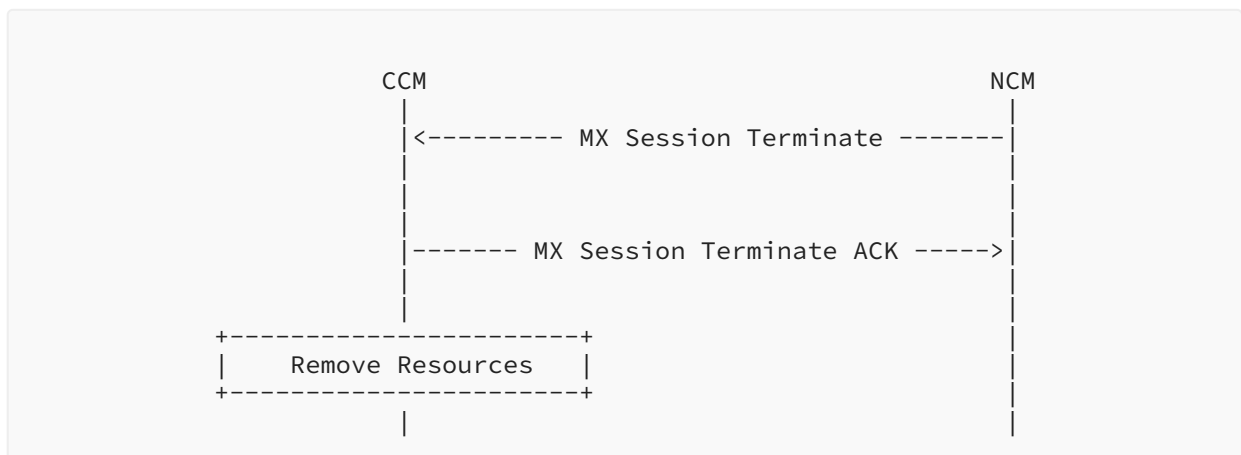
Figure 14: MAMS Session Termination Procedure - Initiated by Network
