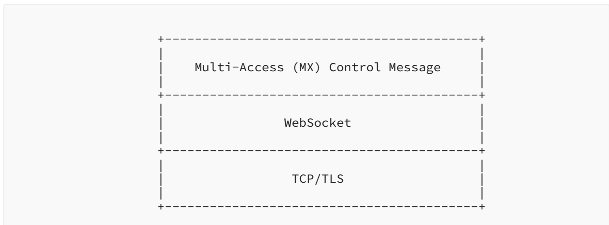
Figure 2: TCP-Based MAMS Control-Plane Protocol Stack
