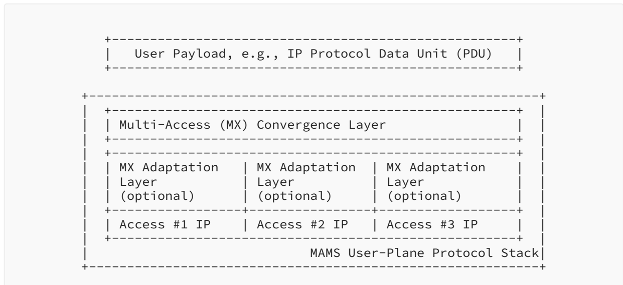
Figure 3: MAMS User-Plane Protocol Stack
