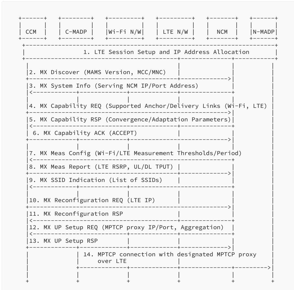
Figure 18: MAMS-Assisted MPTCP Proxy as User Plane - Initial Setup with LTE Leg
