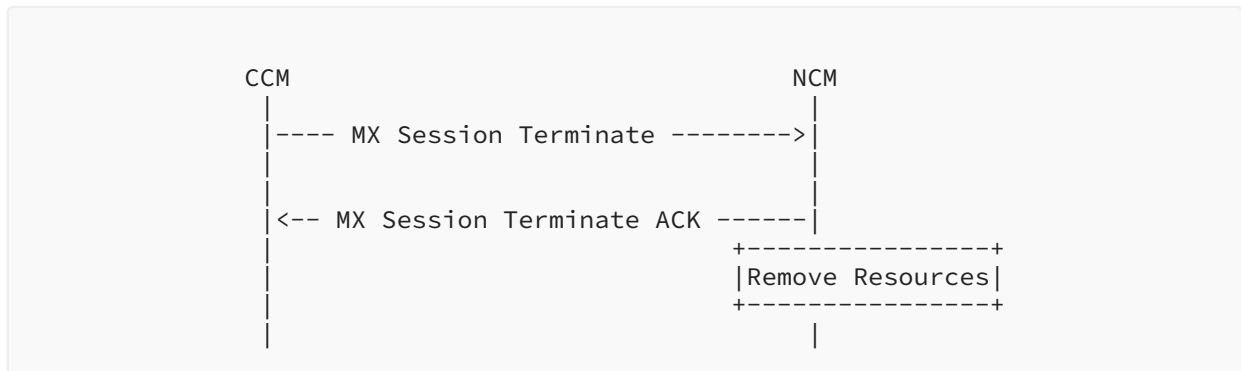
Figure 13: MAMS Session Termination Procedure - Initiated by Client
