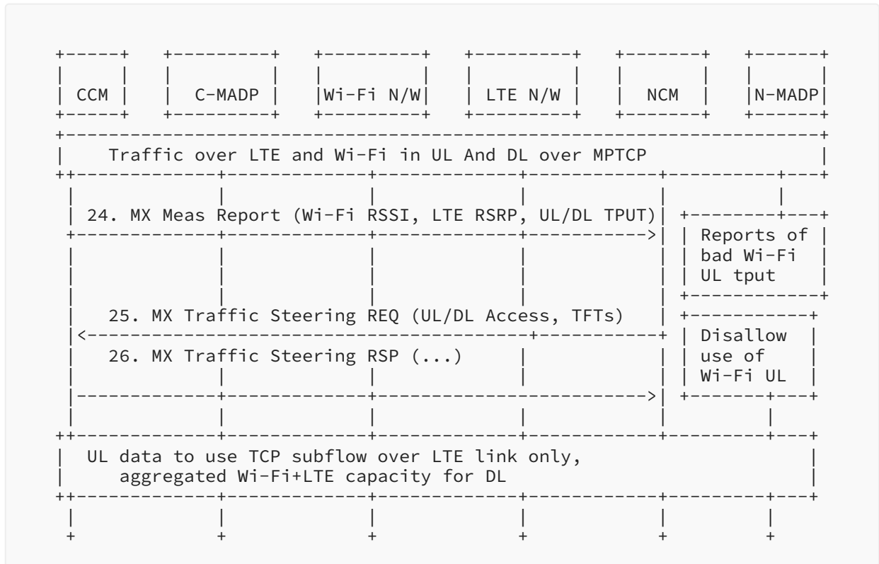
Figure 20: MAMS-Assisted MPTCP Proxy as User Plane - Wi-Fi UL Degrades
